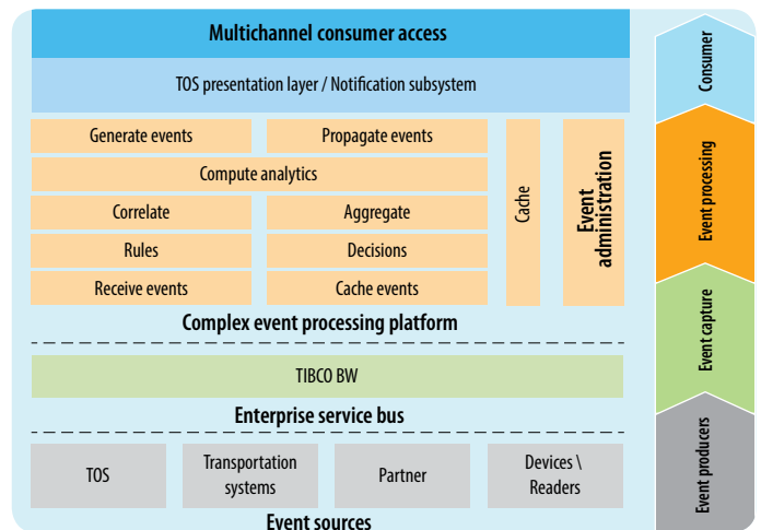
Modernized reference architecture
