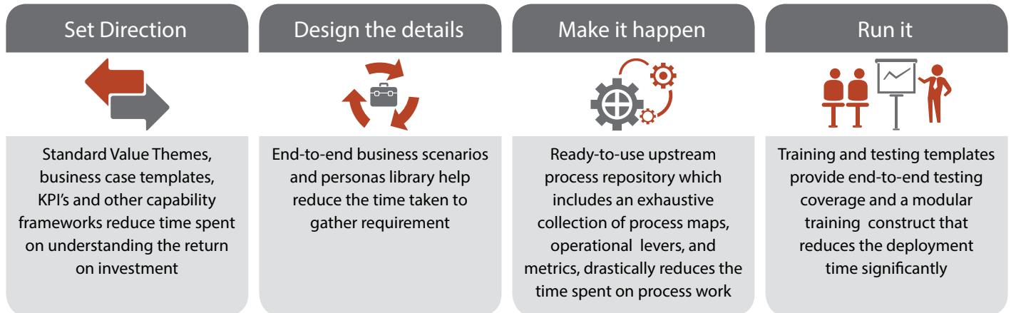
Figure 2: Infosys Accelerators
