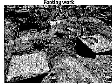
Footing work
